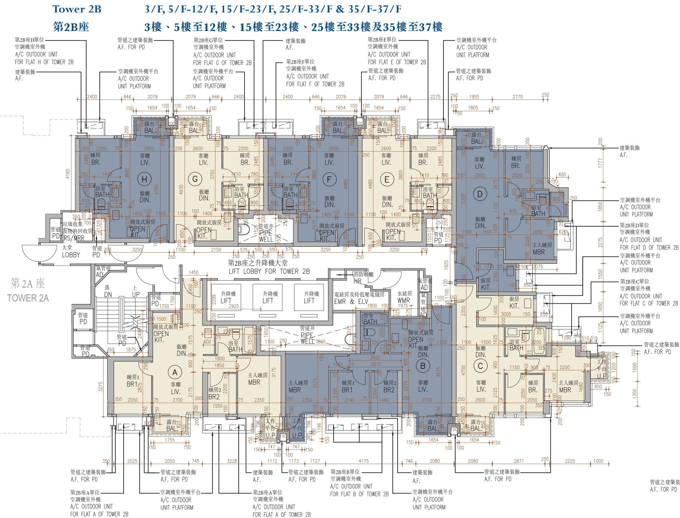
FLOOR PLAN OF FLAT B ON 28/F OF TOWER 2B
